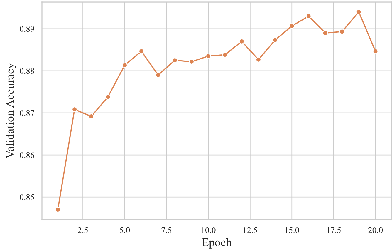
Validation Accuracy vs Epoch
